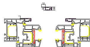
Aluminiumsystem MRS – 12 × 10 mm
